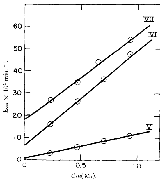
Fig. 4.—Plot of the observed pseudo-first-order rate constants ( k_{obs} ) vs. total imidazole concentration for the hydrolysis of esters V, VI and VII at 70° in 50% dioxane-water (v./v.) and at a pH meter reading of 7.12.
