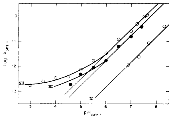
Fig. 3.—pH-rate profiles (60°) for the hydrolysis of the dichloroacetyl esters V, VI and VII in water ( \mu = 1.0 M ). Associated \Delta H^* and \Delta S^* values have been determined and are recorded in Tables II, III and IV.
