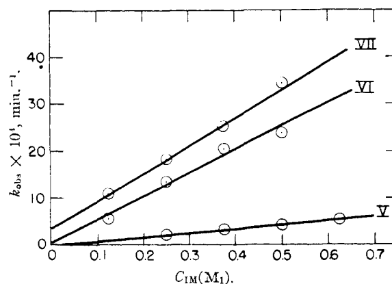
Fig. 5.—Plots of the pseudo-first-order rate constants vs. total imidazole concentration for the hydrolysis of esters V, VI and VII at 30° in 50% dioxane-water (v./v.) and at a pH meter reading of 6.45.
