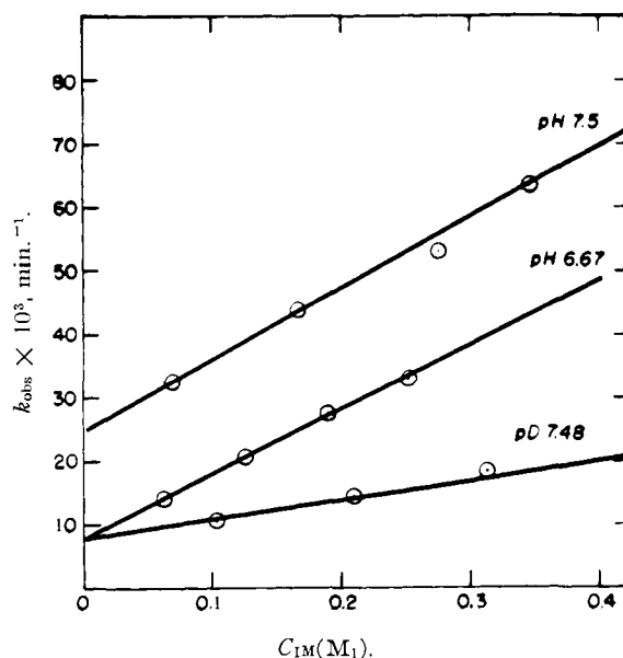
Fig. 2.—Plots of the observed pseudo-first-order rate constants ( k_{obs} ) for the hydrolysis of vic-trans -hydroxycyclopentyl dichloroacetate vs. the concentration of imidazole free base ( C_{IM} ) in water at 30^\circ ( \mu = 1.0 M ) at pH 7.5 and 6.67 and in deuterium oxide at 30^\circ and pD 7.48.
