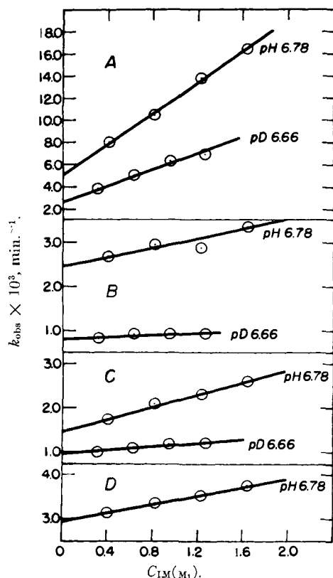
Fig. 1.—Plots of the determined pseudo-first-order rates ( k_{obs} ) of hydrolysis against the concentration of imidazole free base ( C_{IM} ) for reactions studied in H_2O and D_2O : A, 2,2-dichloroethyl acetate; B, monoacetyl pentaerythritol; C, 2-methoxyethyl acetate; D, 2-chloroethyl acetate.
